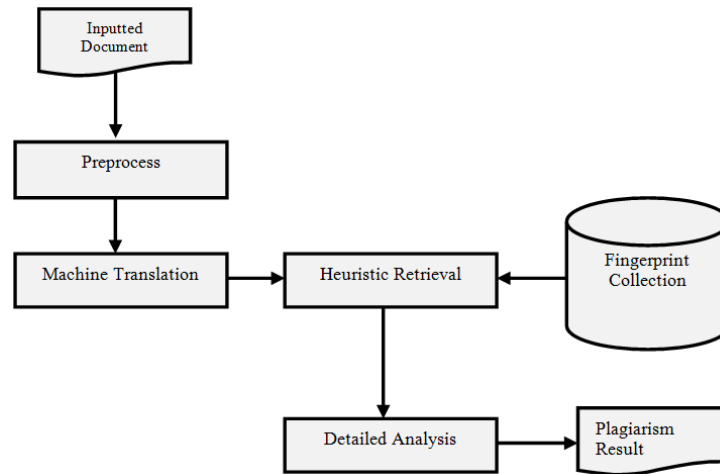
Figure 4. The architecture of the detection system.
