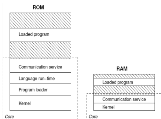
Figure 2. Contiki system.
