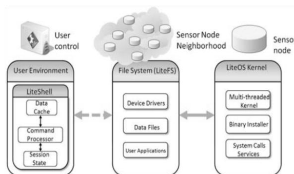
Figure 3. LiteOS architecture.
